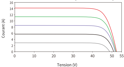
Courbe Courant-Tension (72HL4-BDV 590W)
