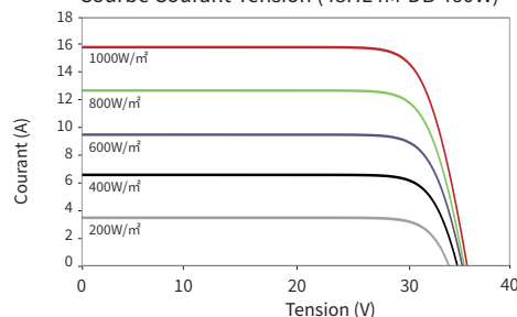
Courbe Courant-Tension (48HL4M-DB 460W)
